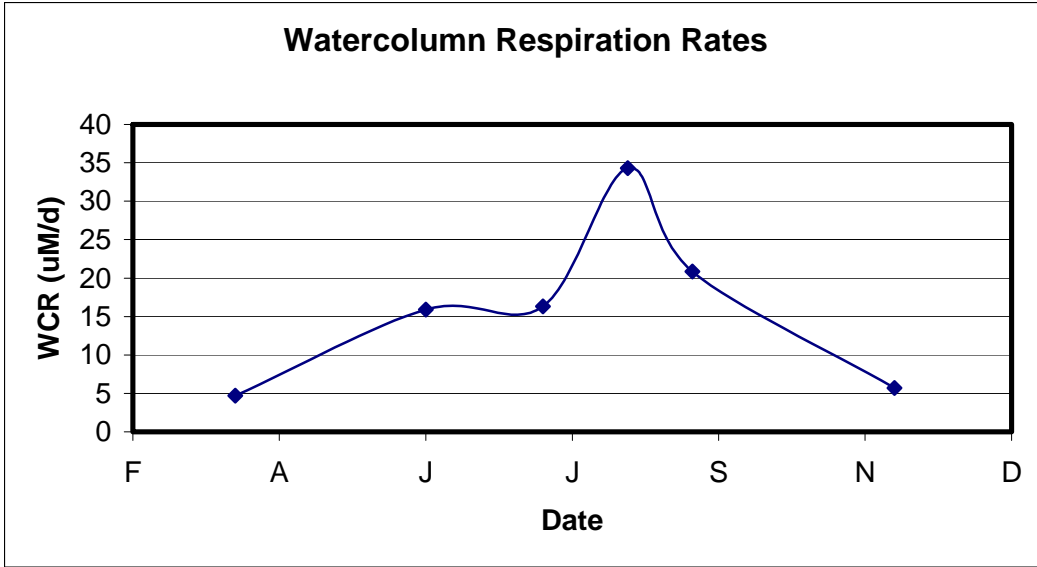
Figure VII-1. Average watercolumn respiration rates (micro-Molar/day) from water collected throughout the Popponneset Bay System at the stations shown in Figure VII-11 (Schleizinger and Howes, unpublished data). Rates vary ~7 fold from winter to summer as a result of variations in temperature and organic matter availability.
