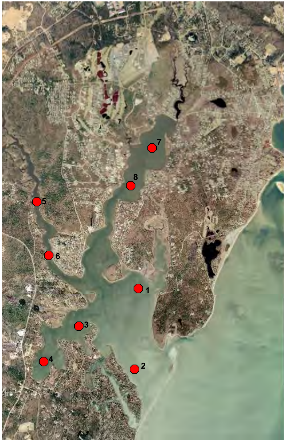
Figure VII-11. Aerial photograph of Popponesset Bay showing location of benthic infaunal sampling stations (red symbol).
