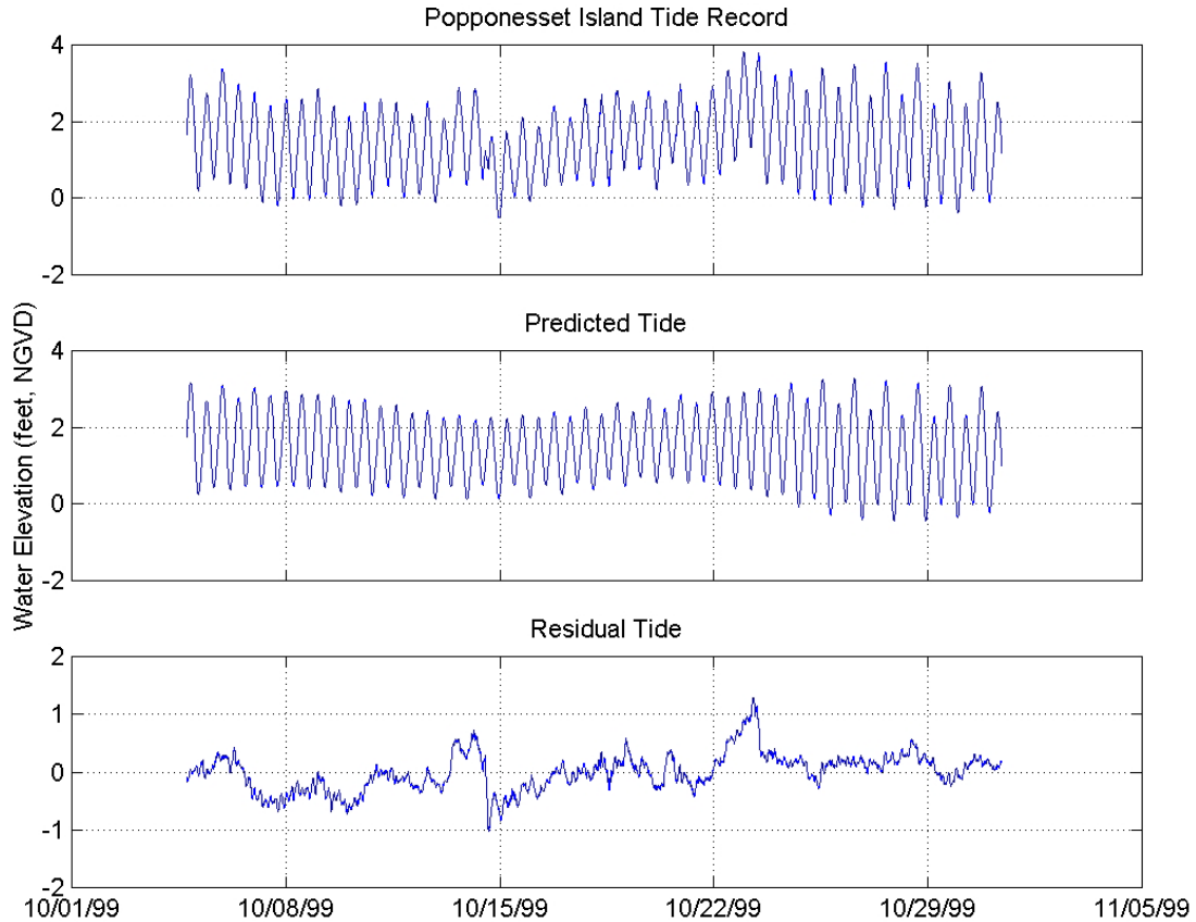
Figure V-10. Results of the harmonic analysis and the separation of the tidal from the non-tidal, or residual, signal measured at Popponesset Island.
