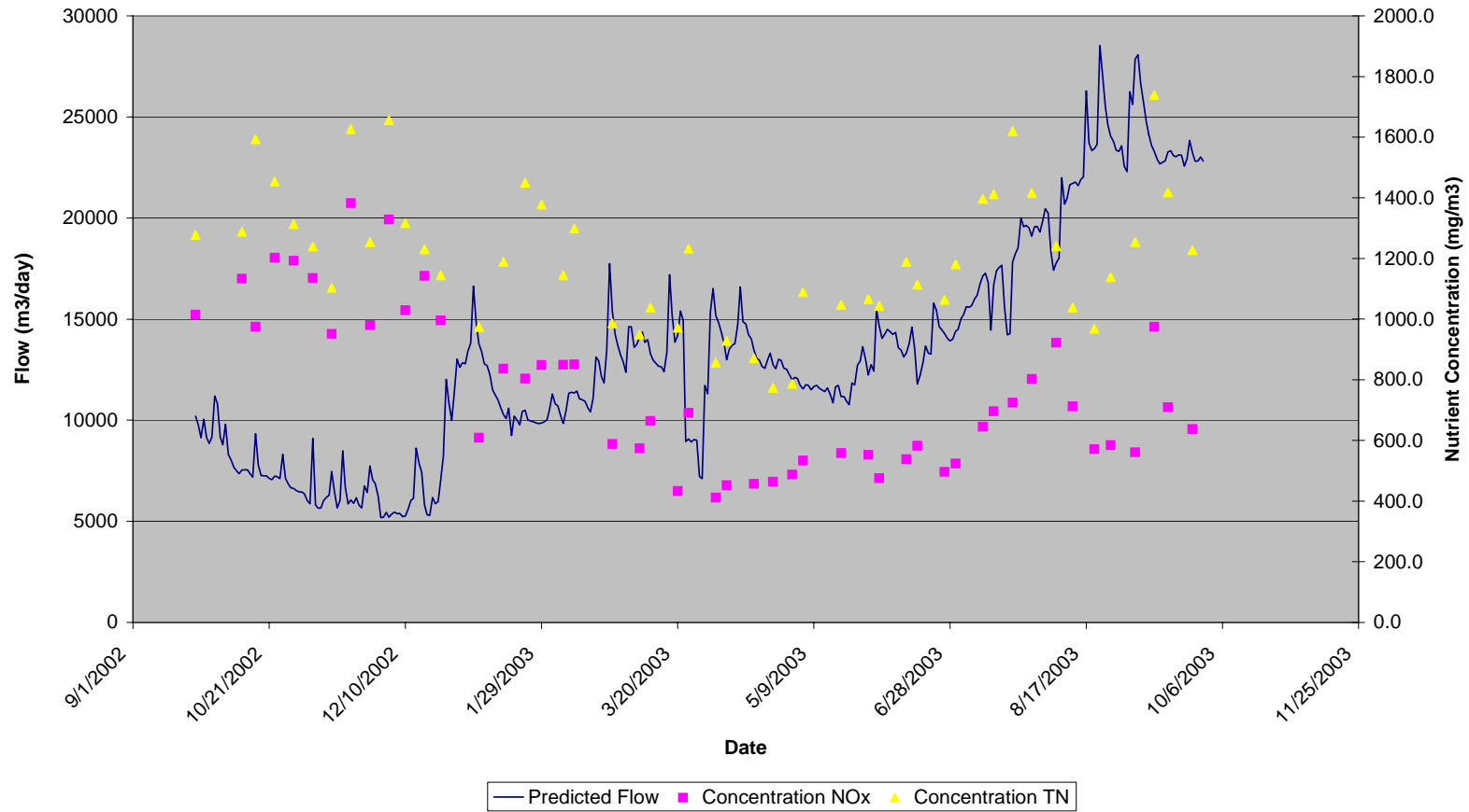
Figure IV-9. Santuit River annual discharge developed from a stream gauge maintained in the outflow from Santuit Pond discharging to Shoestring Bay. Nutrient samples (Nox – Nitrate+Nitrite) were collected approximately weekly and analyzed for inorganic and organic nitrogen species. These data were used to determine both annual flow and total nitrogen transport for determining nitrogen attenuation (see Table IV-5).
