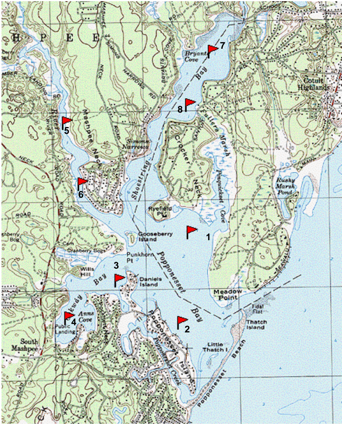
Figure IV-10. Popponesset Bay System locations (red flags) of sediment sample collection for determination of nitrogen regeneration rates. Numbers are for reference in Table IV-9.
