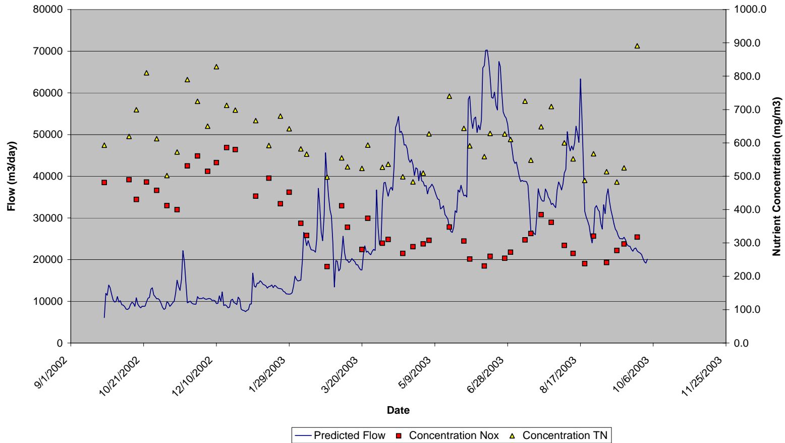
Figure IV-8. Mashpee River annual discharge developed from a stream gauge maintained above the tidal reach of the lower Mashpee River estuarine waters. Nutrient samples (Nox – Nitrate+Nitrite) were collected weekly and analyzed for inorganic and organic nitrogen species. These data were used to determine both annual flow and total nitrogen transport for determining nitrogen attenuation (see Table IV-7).
