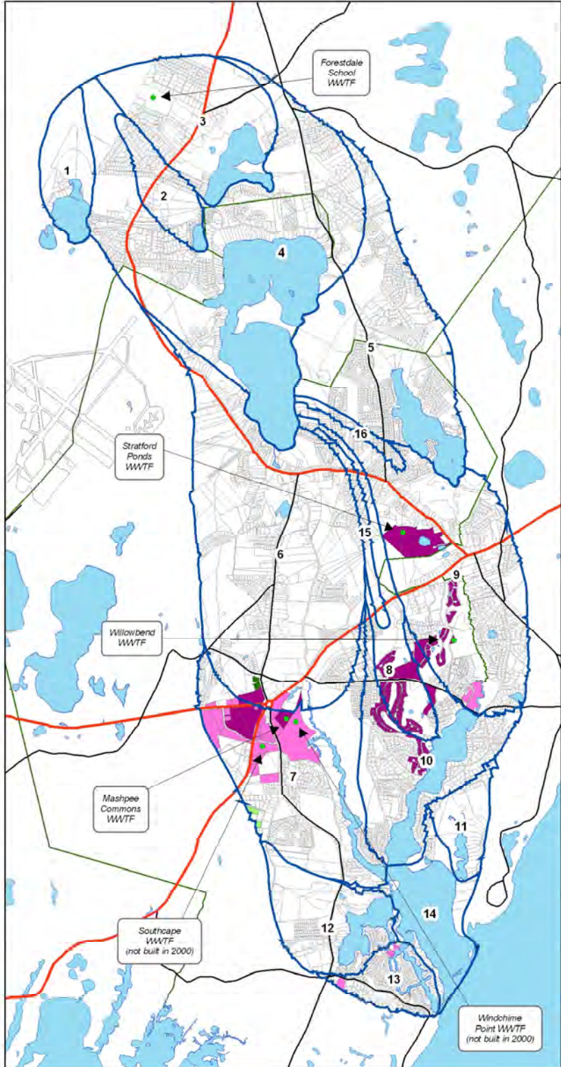
Figure IV-3. Parcels, Parcelized Watersheds, and Private Wastewater Treatment Facilities in the Popponesset Bay watershed.
