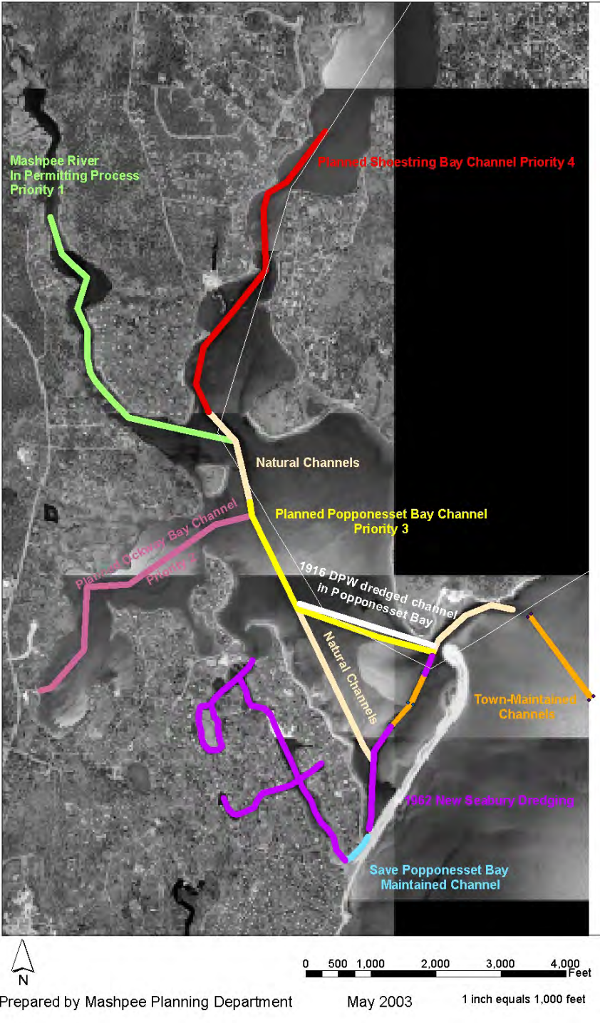
Figure 1: Popponeset Bay Channels (Existing, Dredged and Planned)
